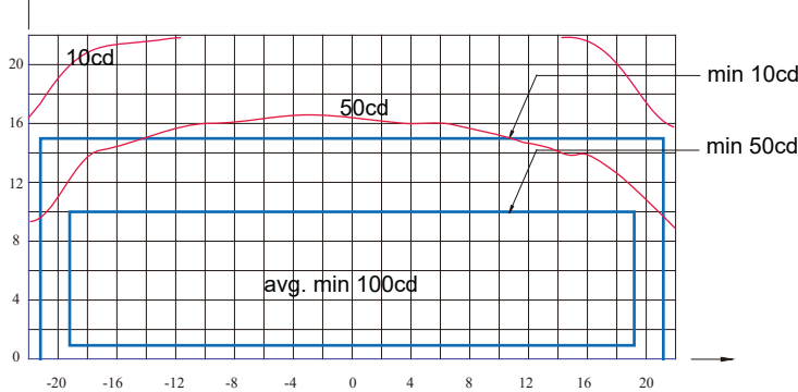
TCLMS-08-S-LED (Green), ICAO Figure A2-12
