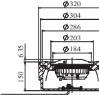
Fig 2. On 12'' shallow base w/ 12''/8'' adapter ring
