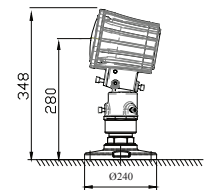
Fig 2. Flange direct mount
